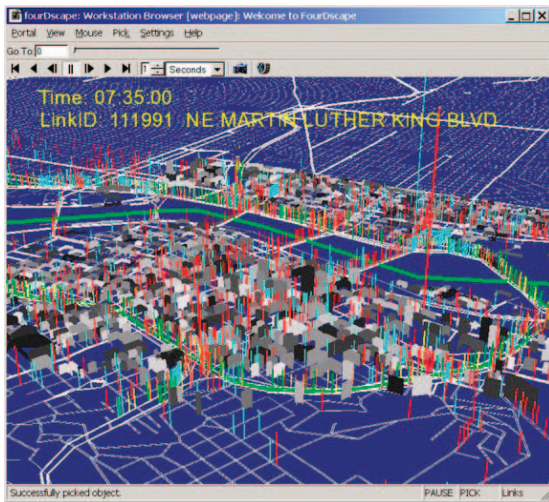
6 Transportation forecasting in downtown Portland, Oregon using Transims and fourDscope. Visualizing simulated traffic patterns enables effective planning, yielding improved transportation infrastructures for predicted traffic volumes. (Image courtesy of Balfour Technologies and IBM Business Consulting)
