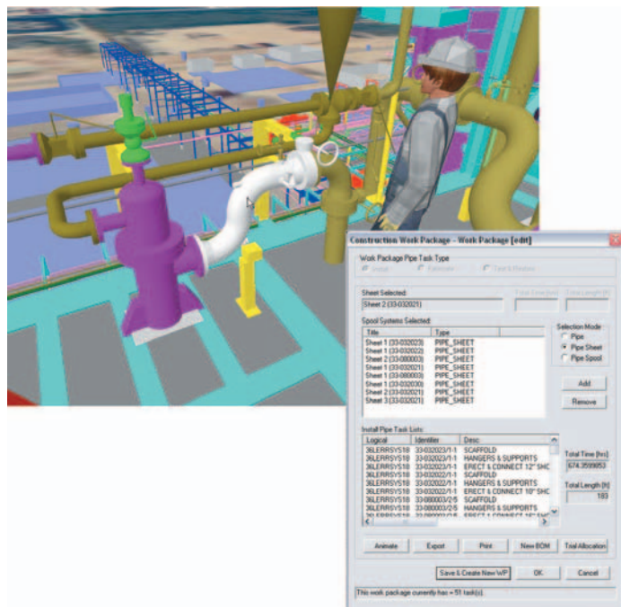
10 ConstructSim displays work package creation where users plans the ideal grouping of materials into work packages creation weeks before mobilizing for these activities in the field. Colors within the picture represent different process systems except for the white spool, which means it’s selected for addition to the work package. (Image courtesy of Reality Capture Technologies)
