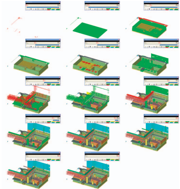
9 Simulation of a construction schedule for a portion of a large-scale semi-conductor facility. Yellow indicates activity in progress, red means critical-path activity, green signifies activity completed. After the activity has completed processing, the geometry changes to its original color. (Image courtesy of CSA)
